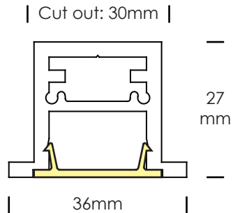
LPLR1M Recessed
