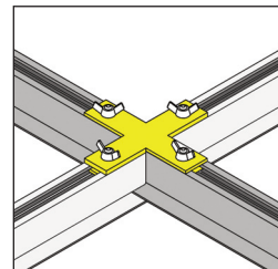
TGRID-CROSS Cross connector. Secures any bars together where they cross.
