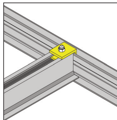
TGRID-CLIP Connector clip to connect either STANDARD- BAR or LIGHT-BAR to the PER-BAR
